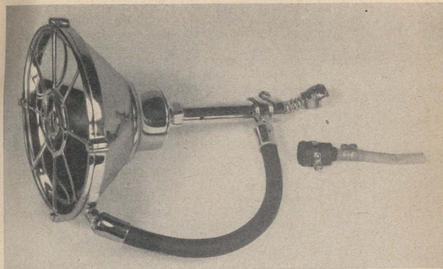
PLATE 52.—Diving light, A. J. Morse & Co. type—Assembled.
