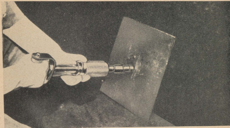
PLATE 105.—Velocity power driver.
