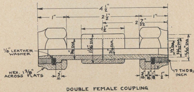
PLATE 32.—Diving air hose double female coupling.
