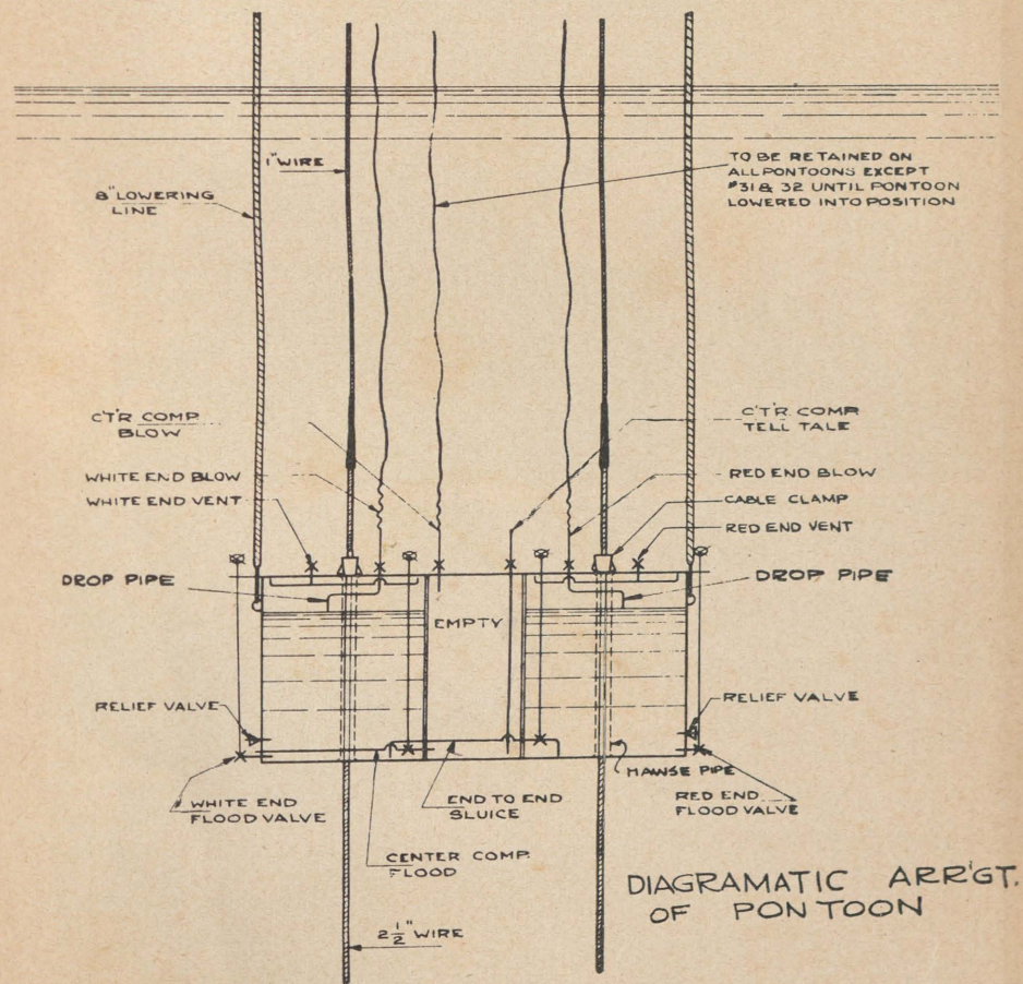
PLATE 102.—Diagrammatic arrangement of pontoon.
