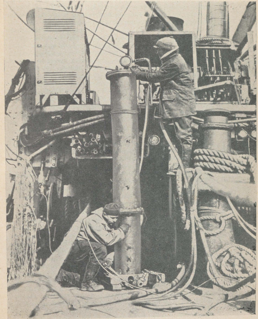
PLATE 109.—Cement gun.
