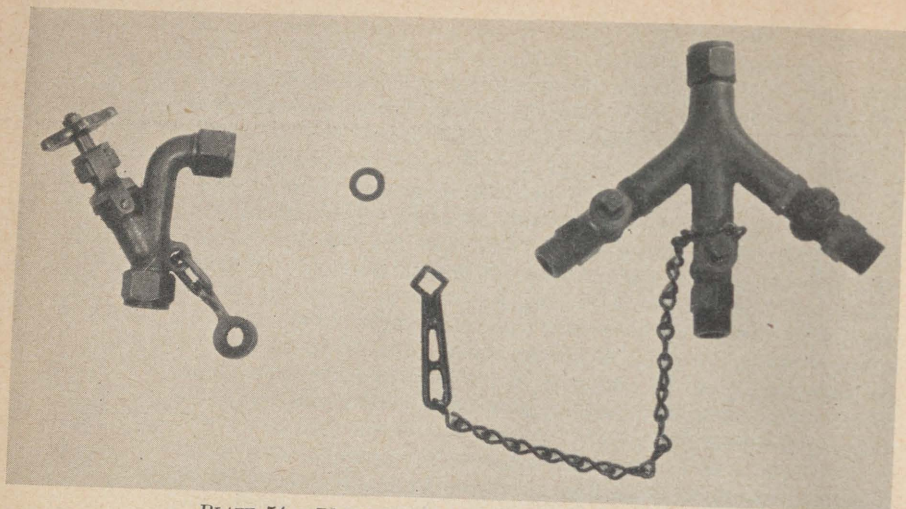
PLATE 54.—Diver's control valve and air manifold.
