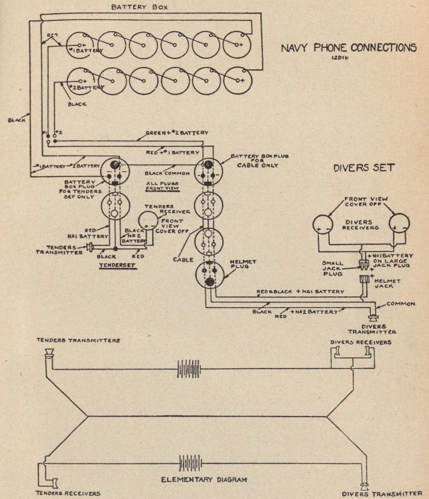
PLATE 73.—Diving telephone, battery type—Wiring diagram for.
