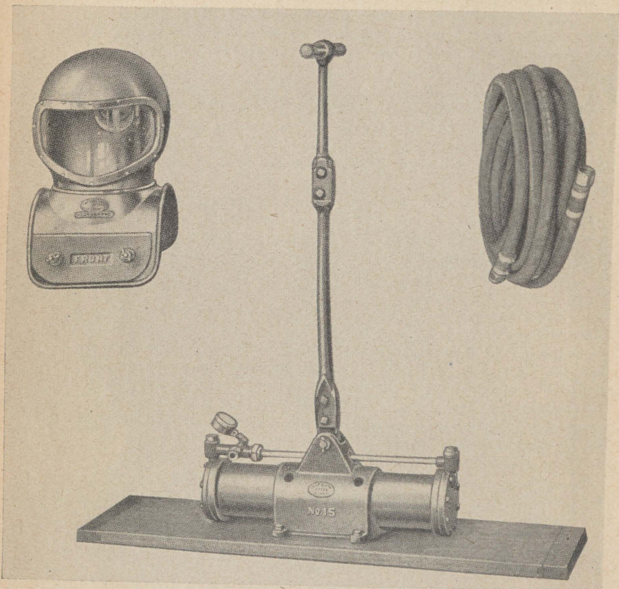
PLATE 77.—Shallow water diving apparatus—A. J. Morse Co. type.
