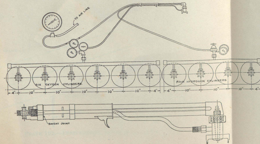
PLATE 103.—Oxy-hydrogen under-water cutting torch.
