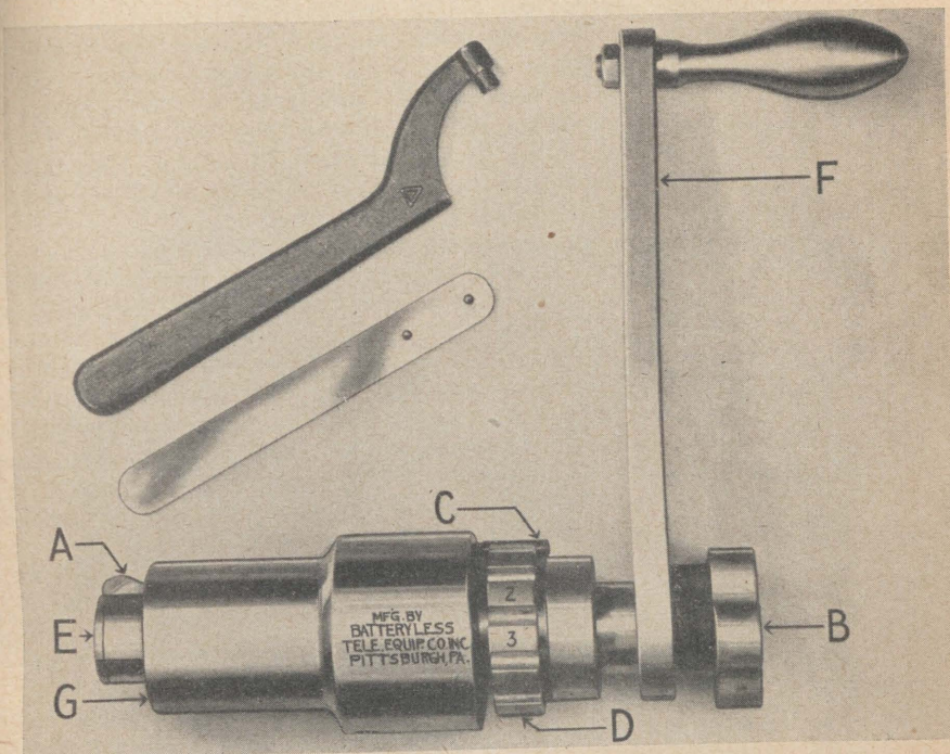
PLATE 28.—Grooving tool for installing air-regulating escape valve.
