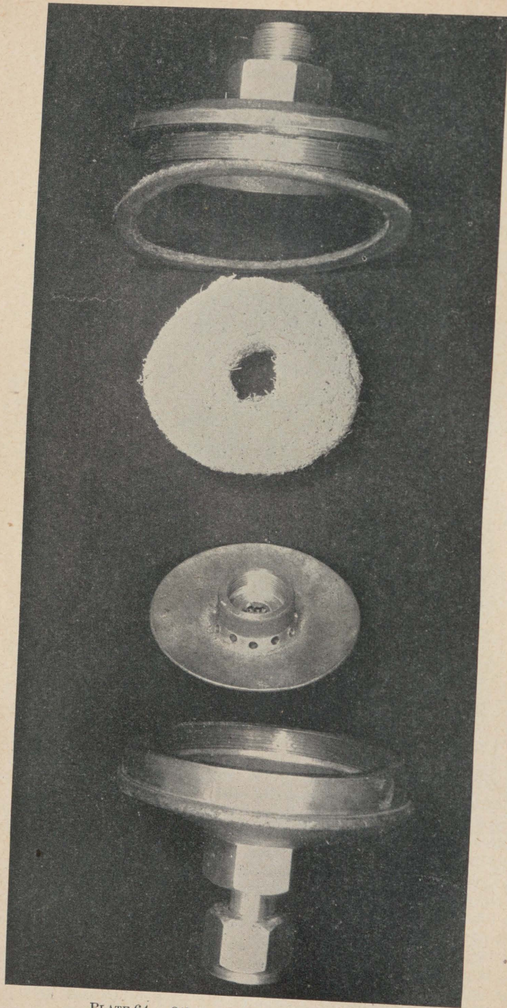
PLATE 64.—Oil Separator—Disassembled.
