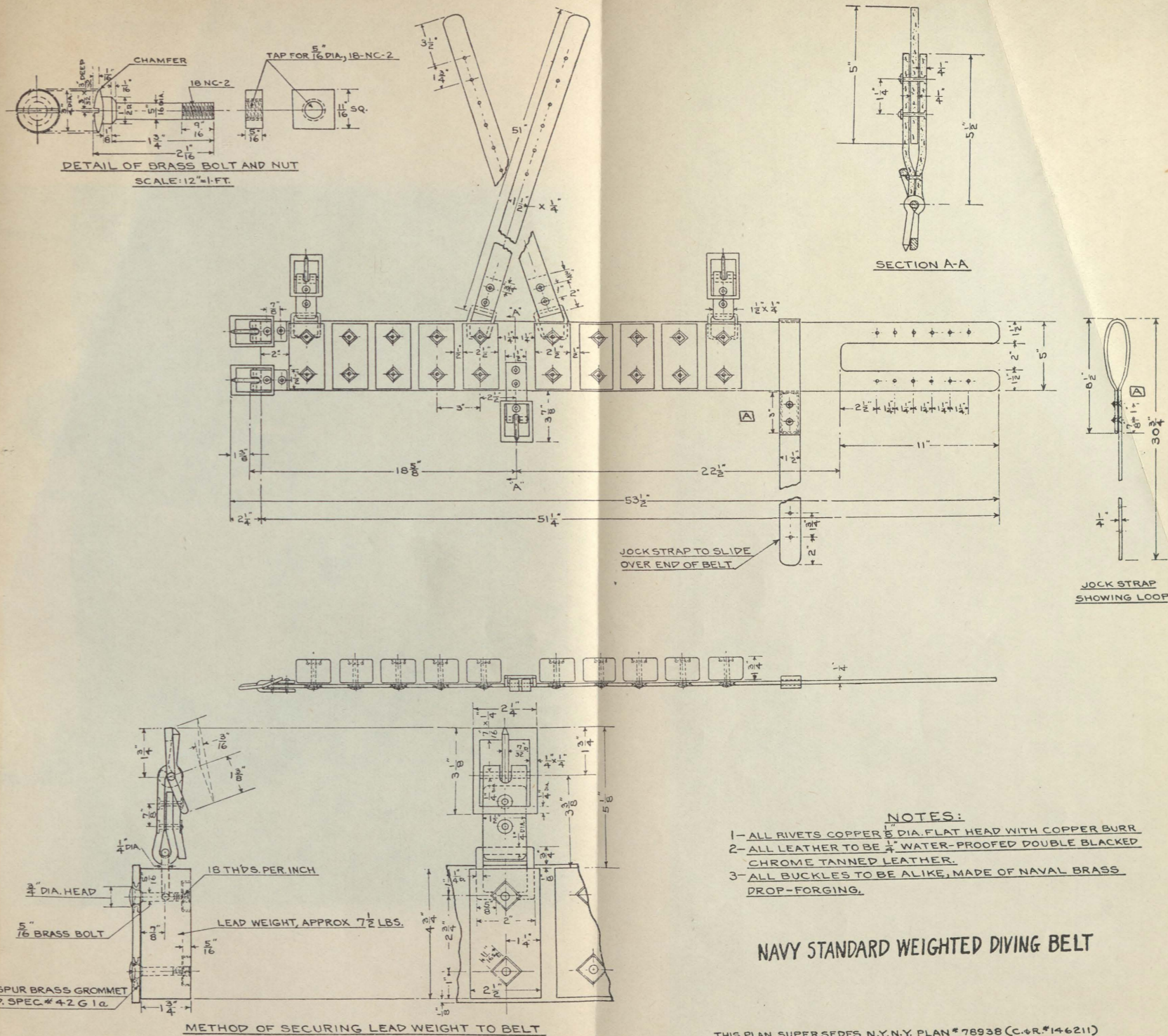
PLATE 11.—Diver's weighted belt.
