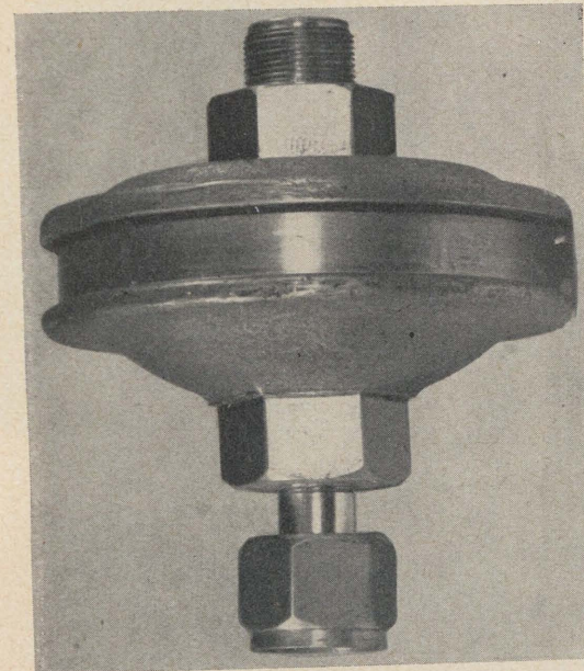
PLATE 63.—Oil separator—Assembled.
