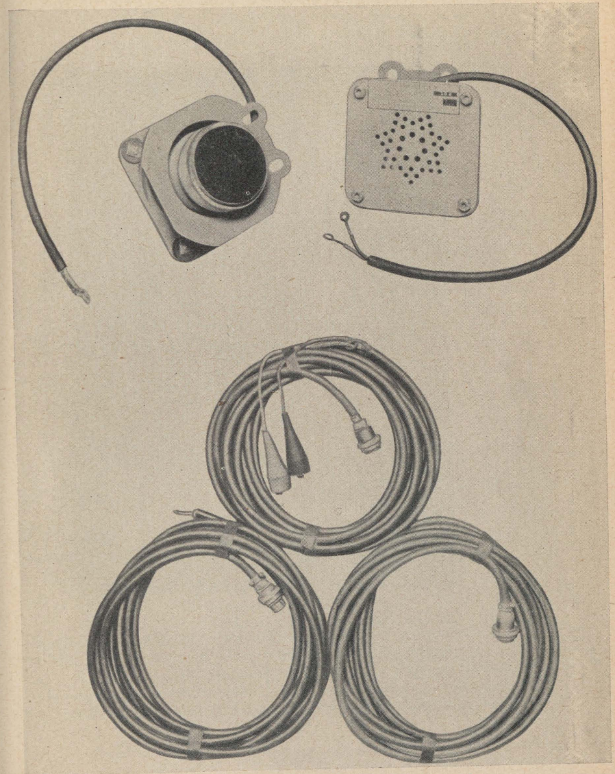
PLATE 73-B.—Diver's reproducer and power cables.
