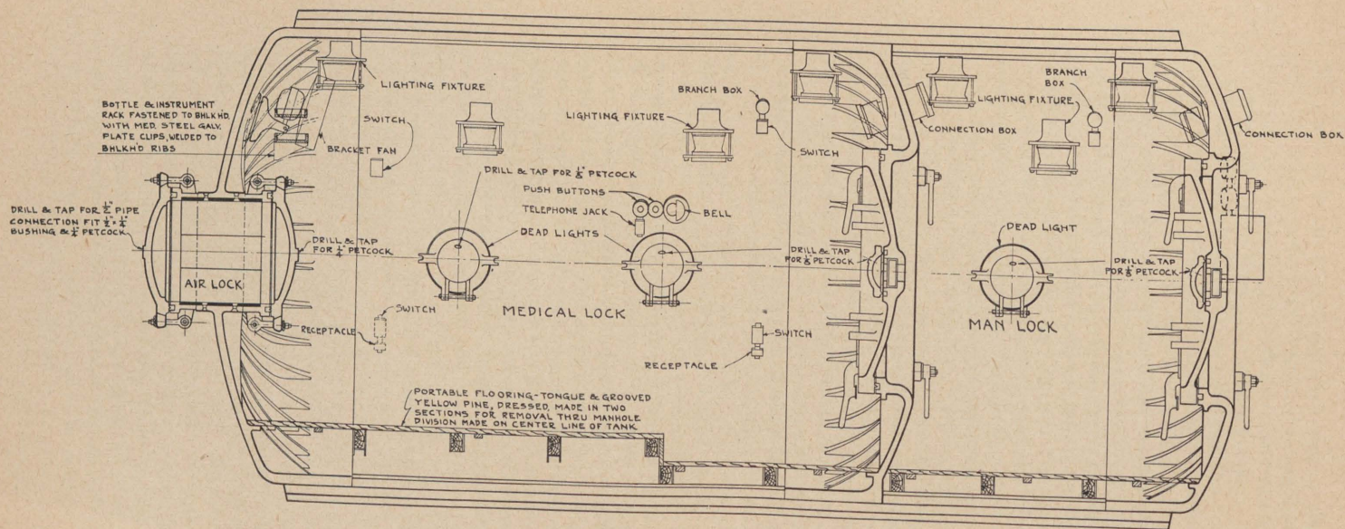
LONGITUDINAL SECTION PLATE 100.—Navy standard recompression chamber.
