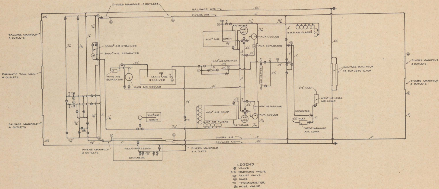
PLATE 101.—Diving and salvage air lines on submarine rescue vessels.
