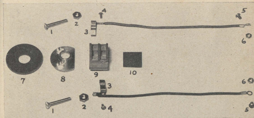
PLATE 71-F.—Diving telephone coupling, for helmet gooseneck (female connection)—Disassembled.
