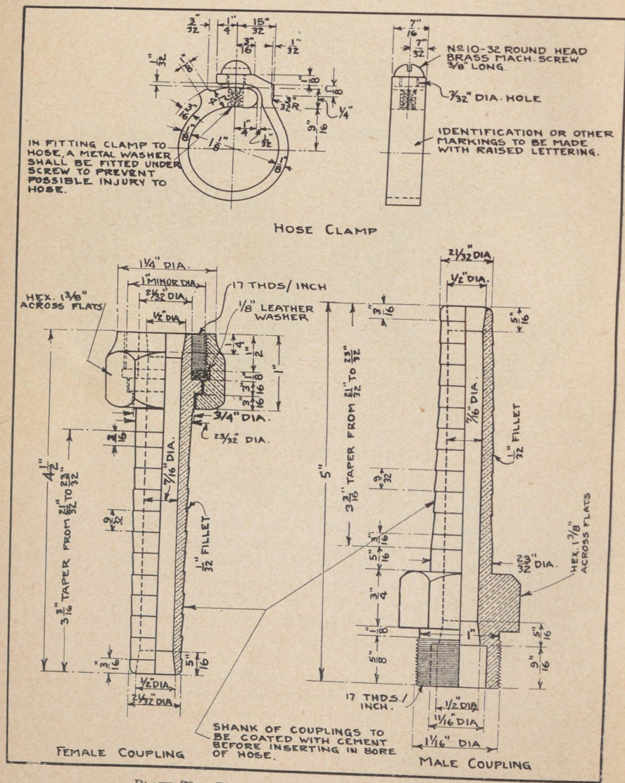
PLATE 30.—Diving air hose couplings and clamps.
