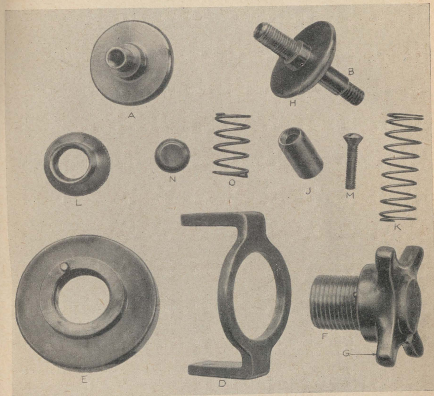
PLATE 27-A.—Helmet, air-regulating escape valve, disassembled.
