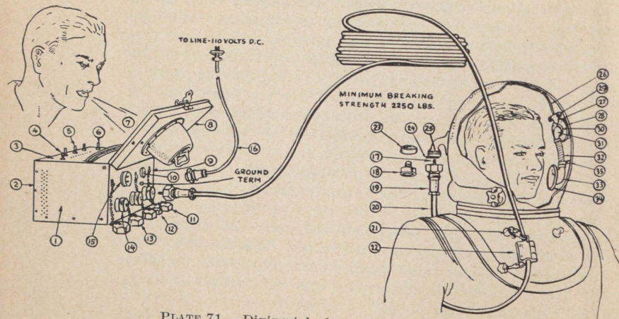
PLATE 71.—Diving telephone, amplifier type.
