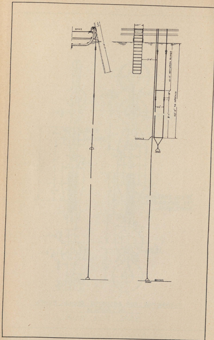
PLATE 84.—Arrangement of diving ladder, decompression stage, and descending line on diving launch.
