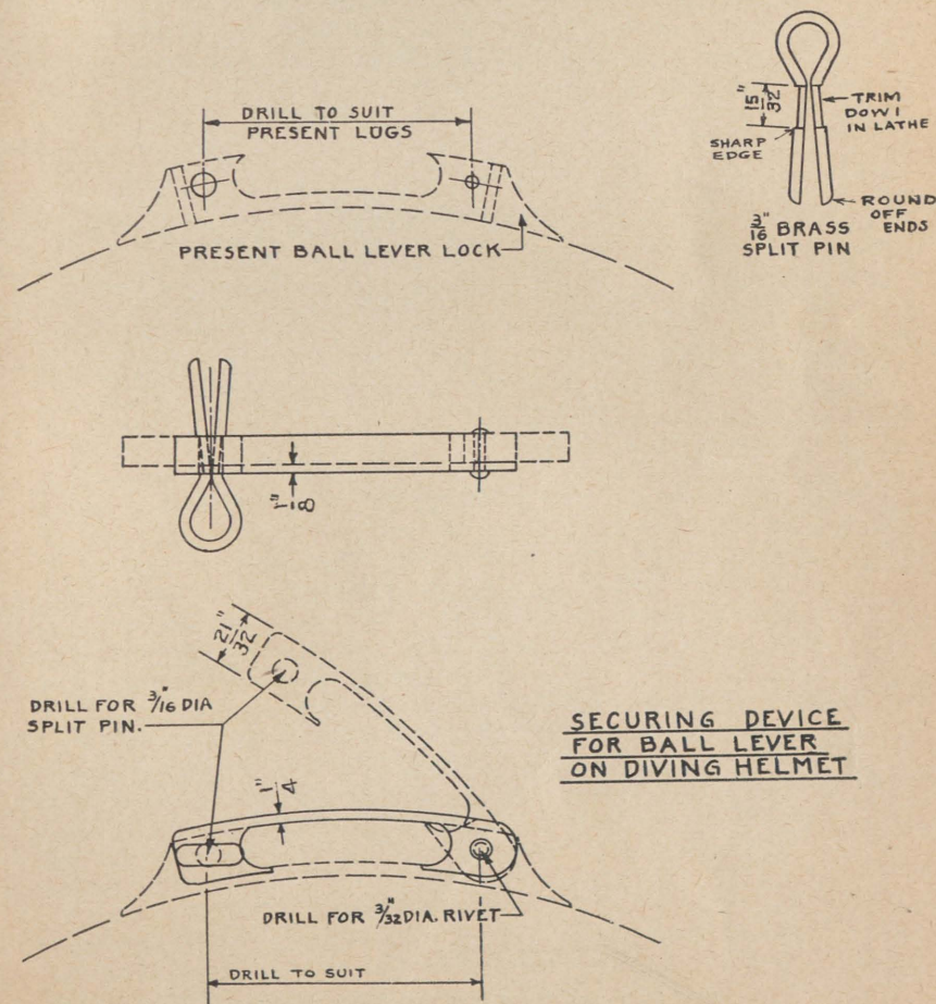
PLATE 25.—Helmet lock.
