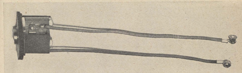
PLATE 71-E.—Diving telephone coupling, for helmet gooseneck (female connection)—Assembled.
