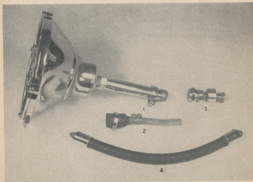
PLATE 53.—Diving light, A. J. Morse & Co. type—Disassembled.
