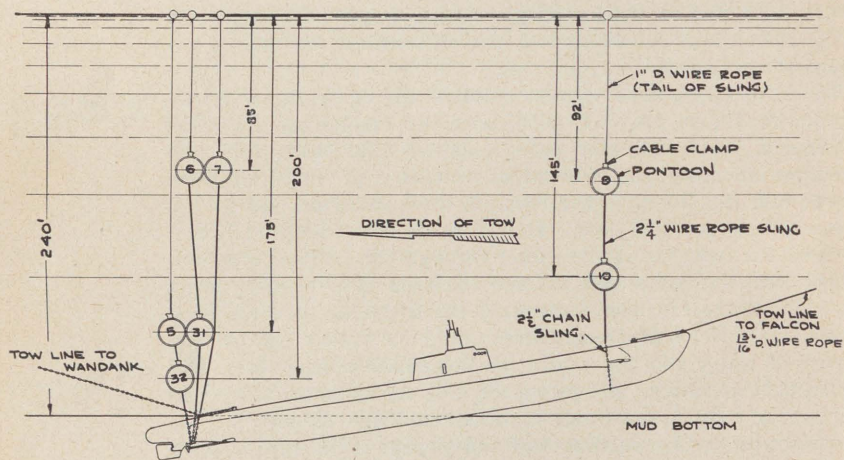
ARRANGEMENT OF PONTOONS LIFT OF 13 JULY, 1939 SCALE: \frac{1}{50}'' = 1'-0''
