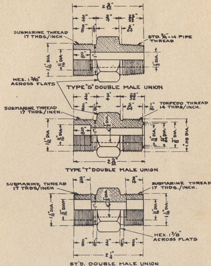
PLATE 31.—Diving air hose special fittings.
