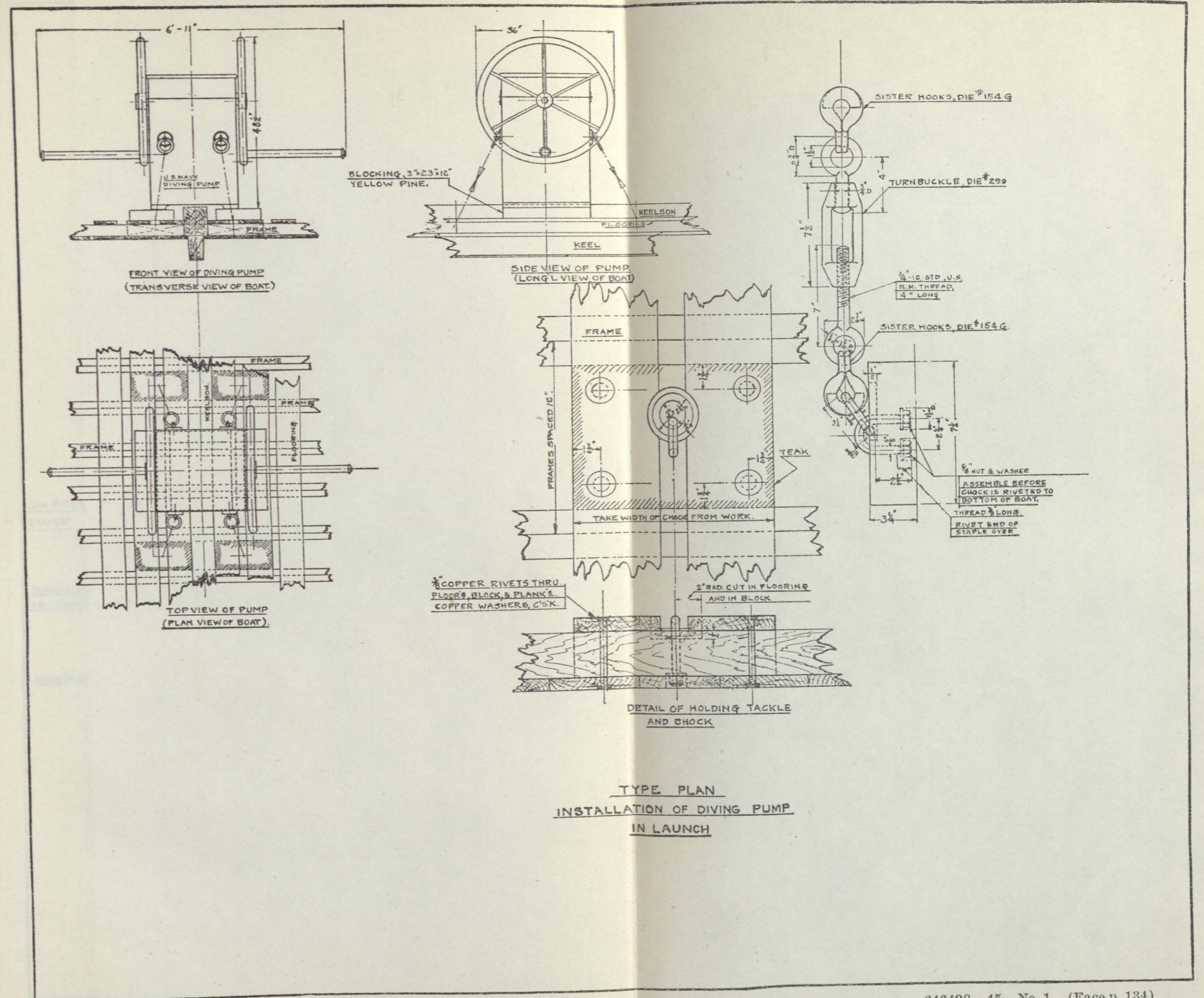
PLATE 83.—Type plan—Installation of diving pump in launch.
