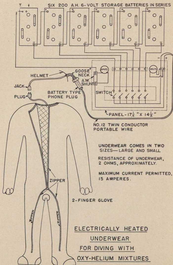
PLATE 90.—Electrically heated undergarments for diving with oxy-helium mixtures.
