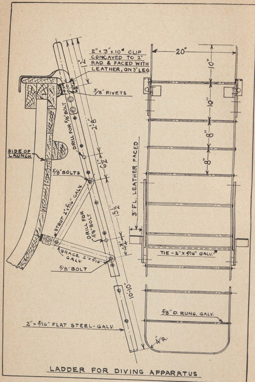
PLATE 34.—Diving ladder.
