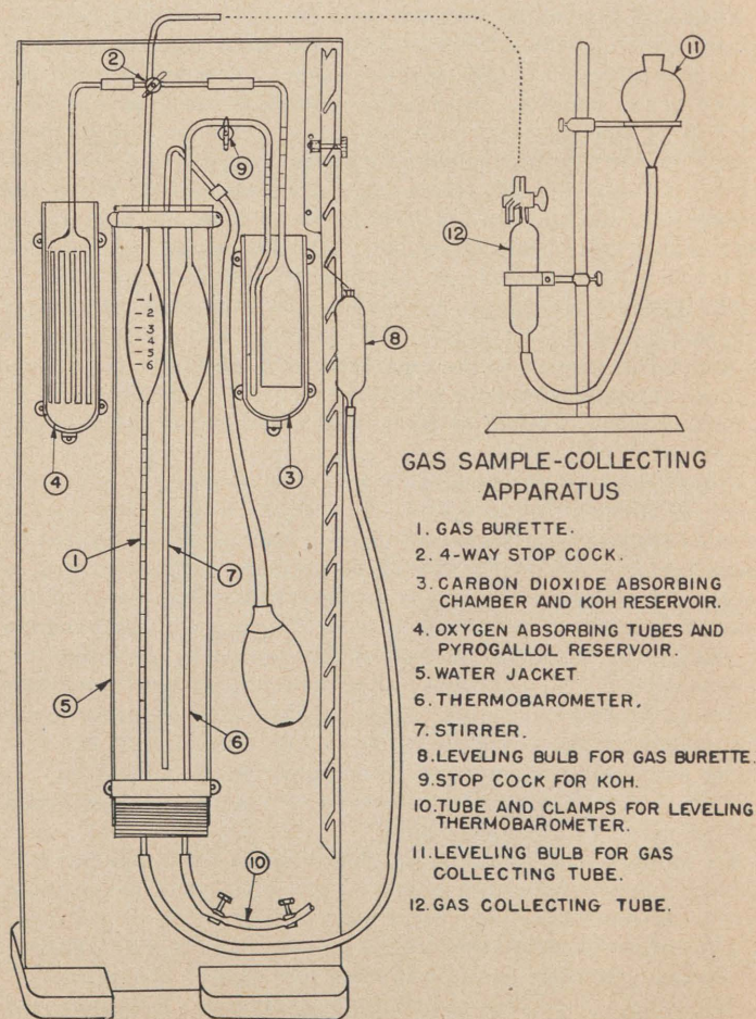
PLATE 91.—Haldane-Henderson gas analysis apparatus.
