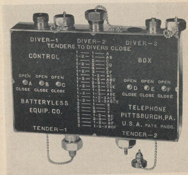
PLATE 70-A.—Diving telephone, batteryless type—Control box.
