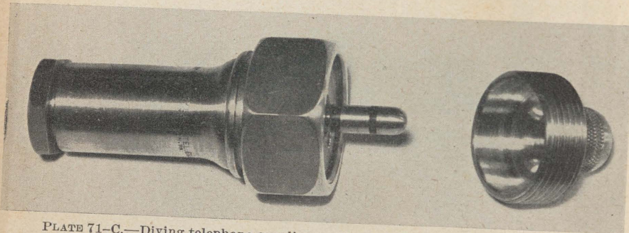
PLATE 71-C.—Diving telephone coupling, male (jack plug housing) — Assembled.
