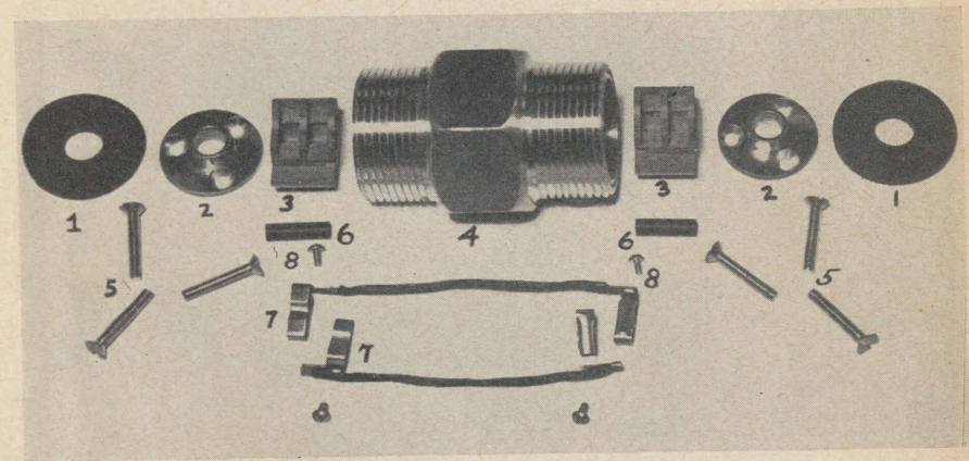
PLATE 71-B.—Diving telephone coupling, double female connection—Disassembled.
