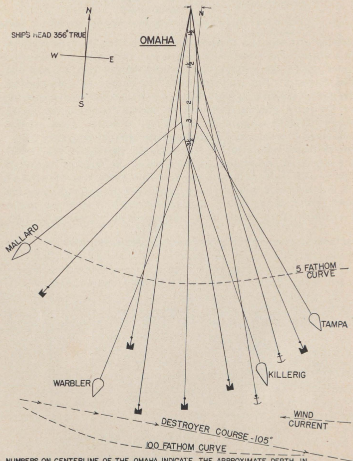
PLATE 113.—Arrangement of salvage gear used on salvage of U. S. S. Omaha .
