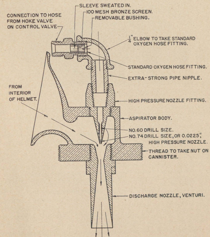
PLATE 97.—Helmet oxygen-helium, cross section of aspirator and discharge nozzle venturi.
