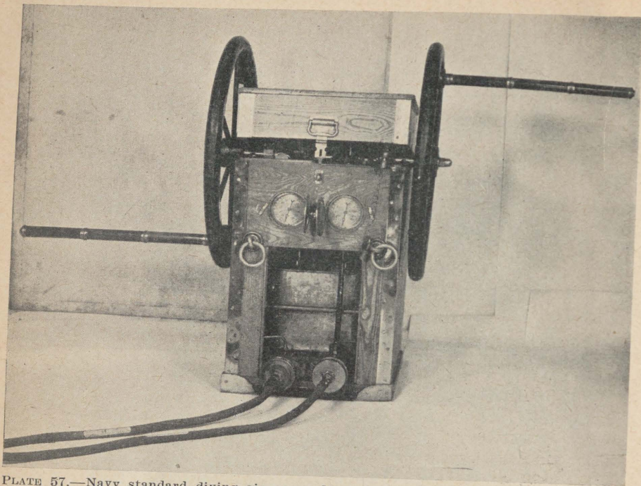
PLATE 57.—Navy standard diving air pump, Mark III, with top raised and front cover removed.
