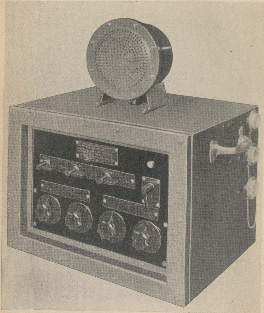
PLATE 73-A.—Amplifier and tender's reproducer—front and right side.
