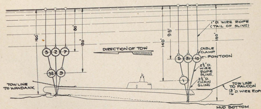
ARRANGEMENT OF PONTOONS LIFT OF 17-AUG, 1939 SCALE: \frac{1}{50}'' = 1'-0''
