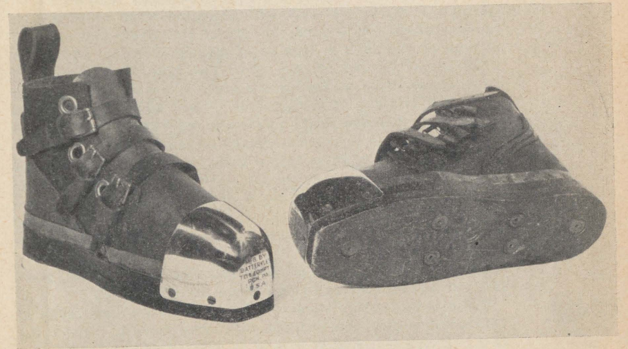
PLATE 65.—Navy standard diving shoes.
