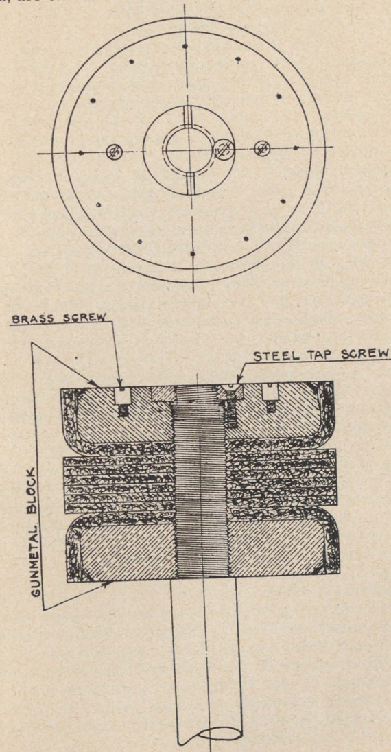
PISTON FOR TWO-CYLINDER DOUBLE-ACTING DIVING AIR PUMP. MARK III
