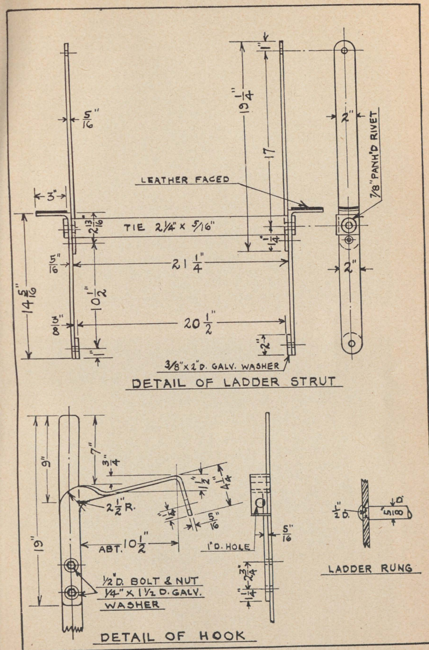
PLATE 35.—Diving ladder details.
