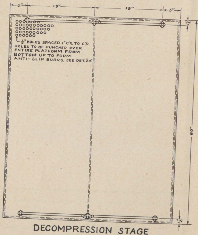
PLATE 68.—Decompression stage, large, plan view.
