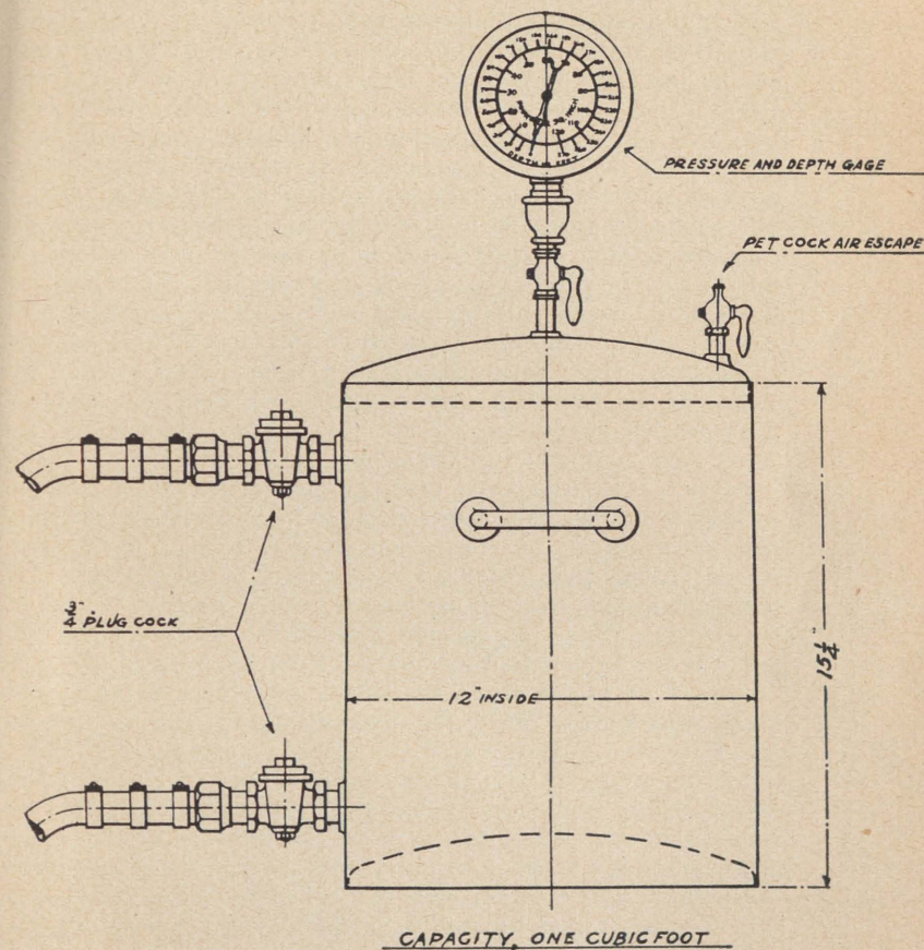
CAPACITY, ONE CUBIC FOOT PLATE 74-A.—Tank, test, for diving air system.
