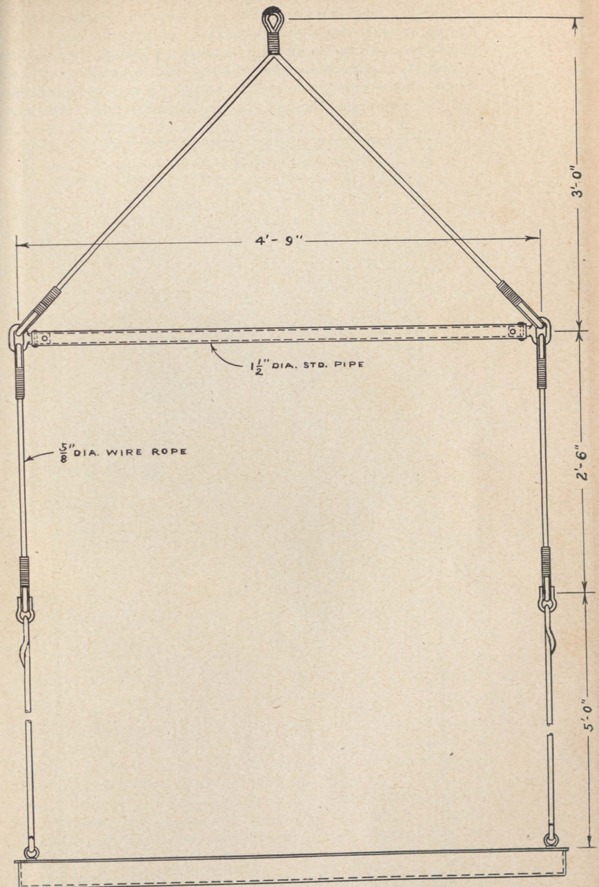
48" x 60" DECOMPRESSION STAGE WITH SUPPORTS
