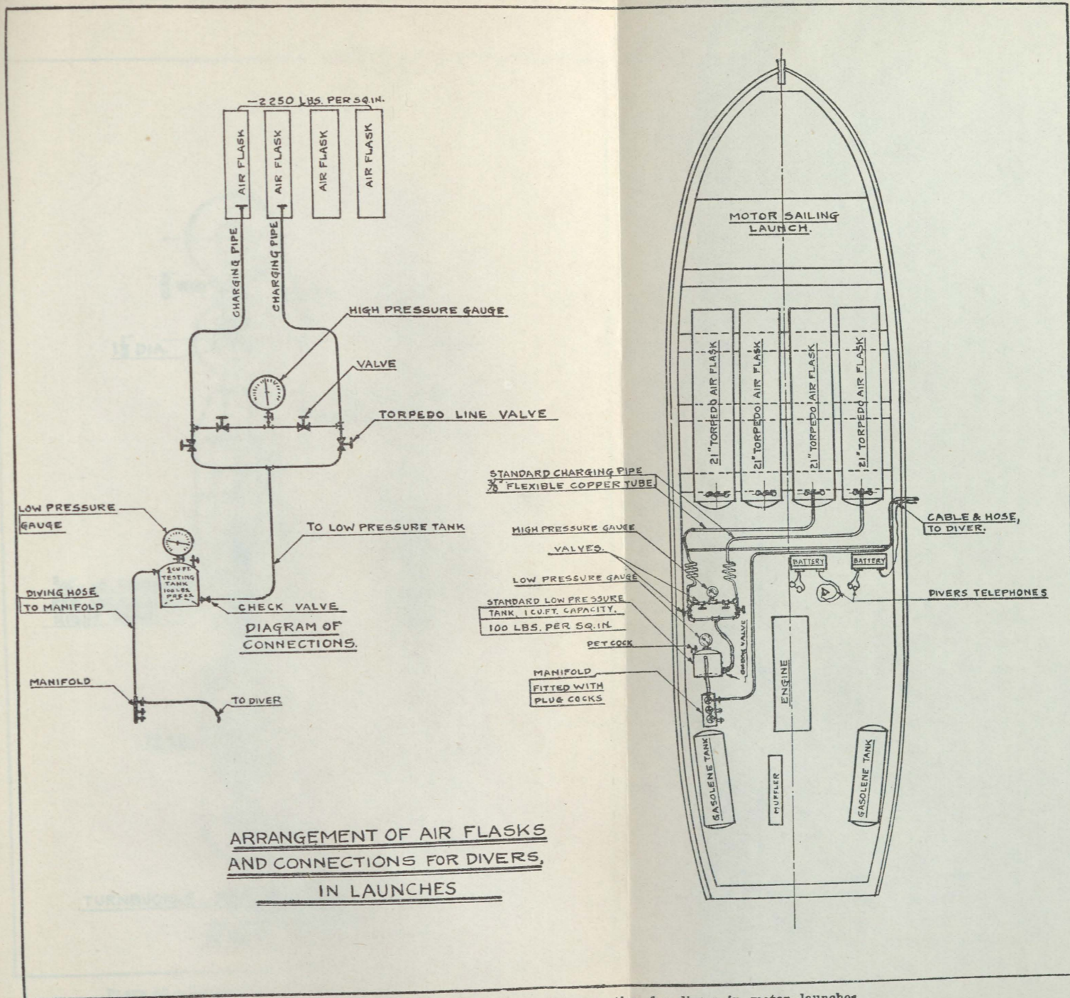
PLATE 85.—Arrangement of air flasks and connection for divers in motor launches. 646428—45—No. 2 (Face p. 134)
