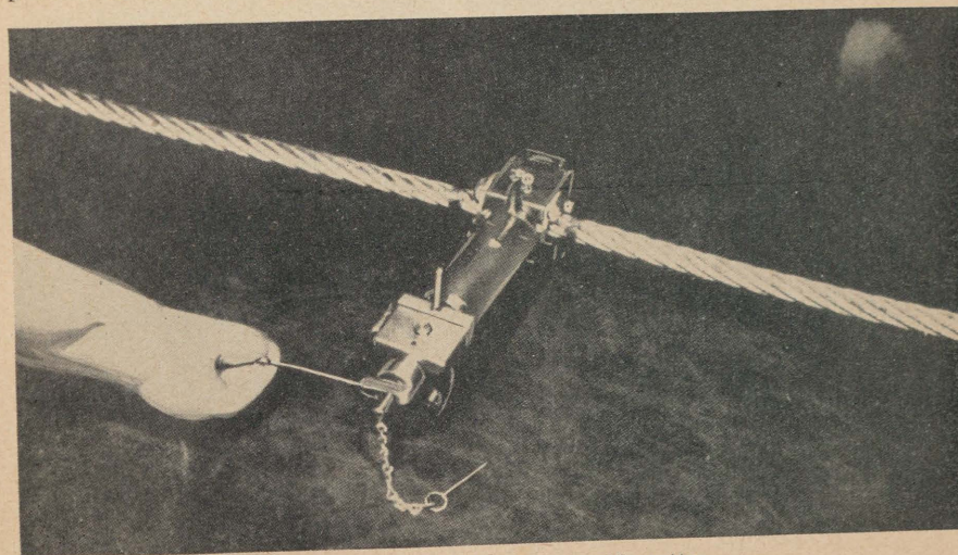
PLATE 106.—Velocity power cable cutter.
