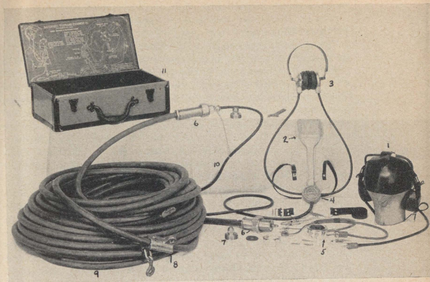
PLATE 70.—Diving telephone, batteryless type.
