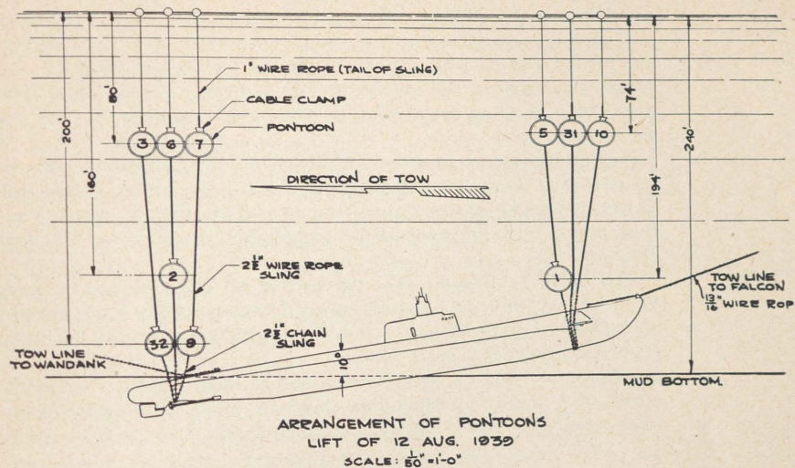
PLATE 111.—Salvage of U. S. S. Squalus —arrangement of pontoons.
