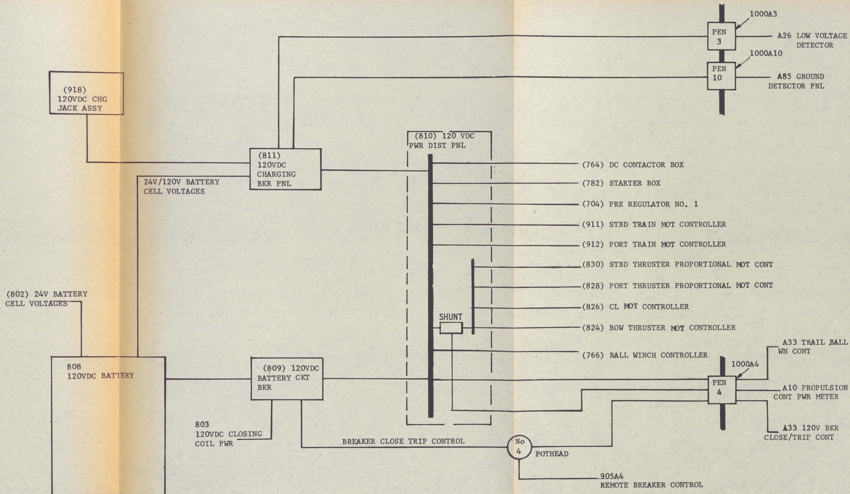
FIGURE 3-2. 120 VDC POWER DISTRIBUTION SYSTEM
