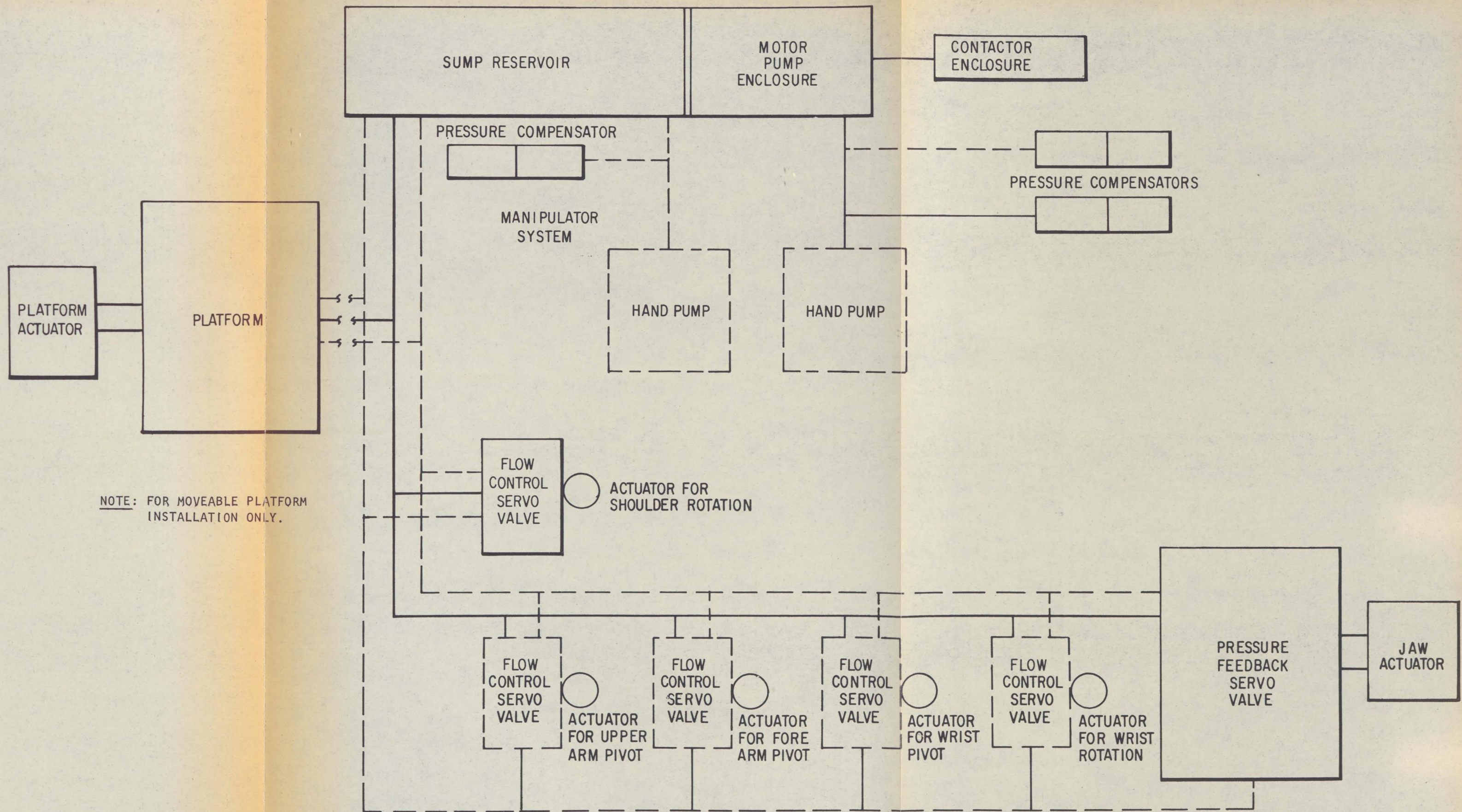
FIGURE 6-2. MANIPULATOR HYDRAULIC BLOCK SYSTEM
