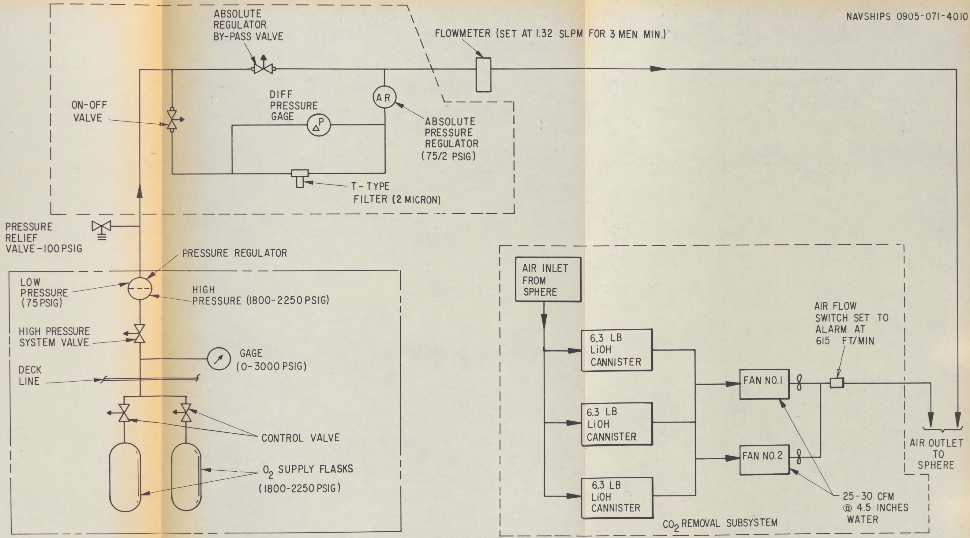
FIGURE 5-2. MAIN O 2 SYSTEM
