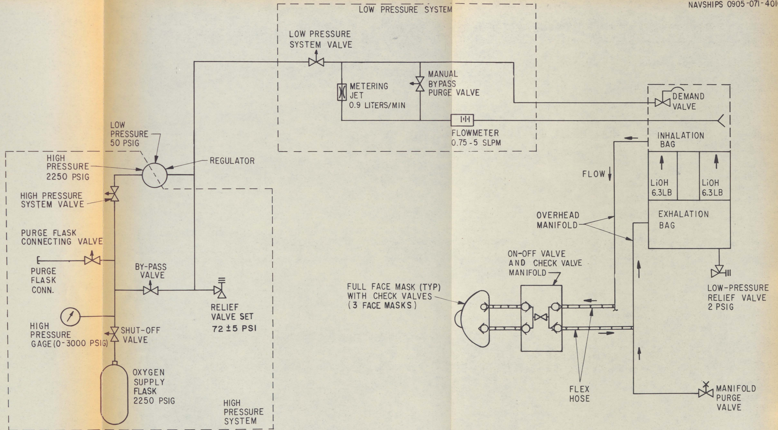
FIGURE 5-3. EMERGENCY O 2 SYSTEM
