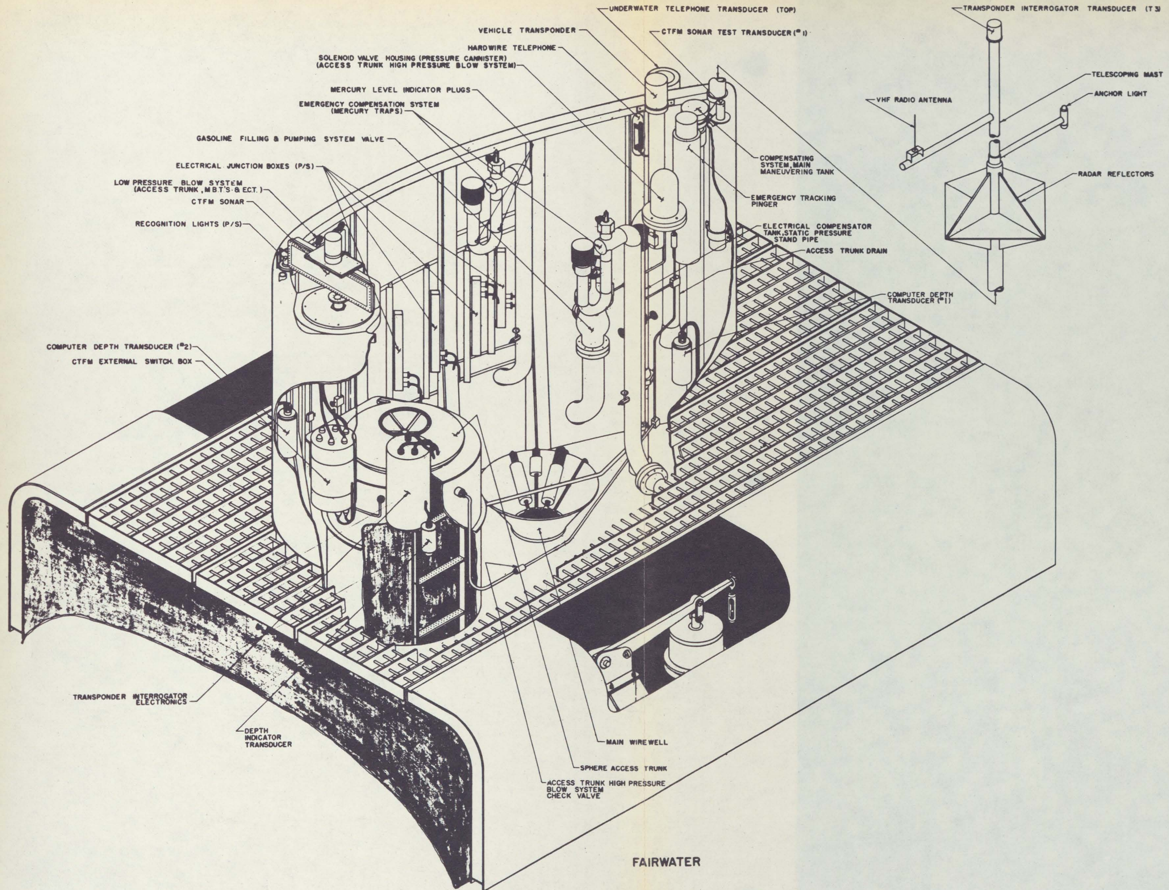
FIGURE 1-4. SAIL EQUIPMENT ARRANGEMENT
