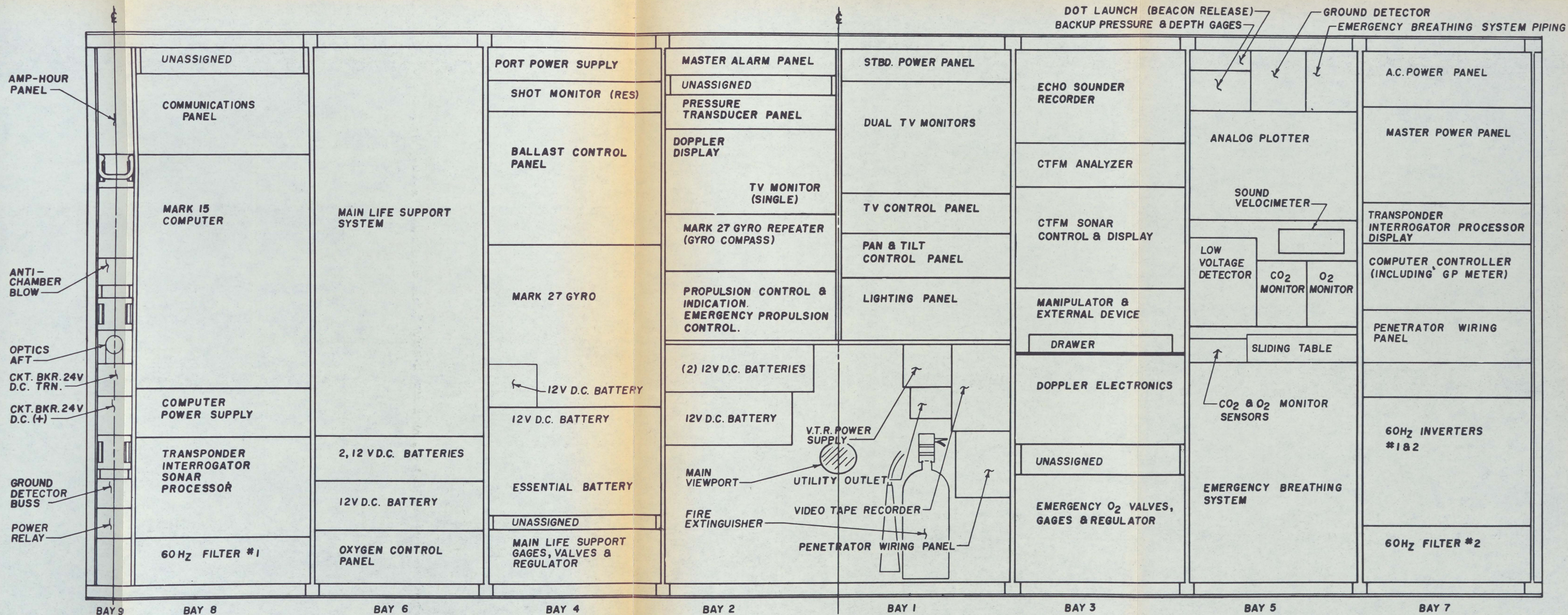
FIGURE 1-6. SPHERE CONTROL AND INSTRUMENT LAYOUT
