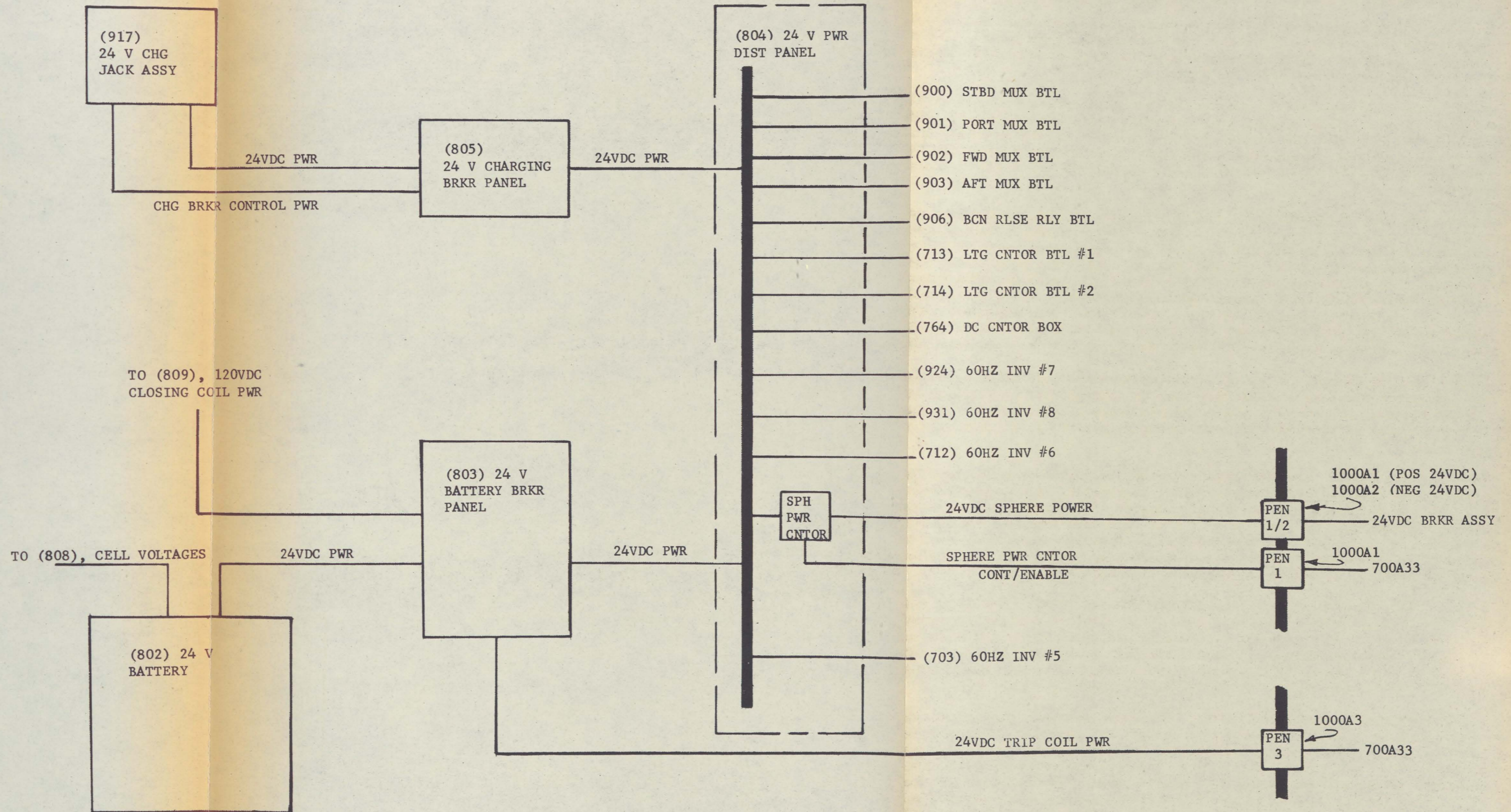
FIGURE 3-1. 24VDC EXTERNAL POWER DISTRIBUTION SYSTEM
