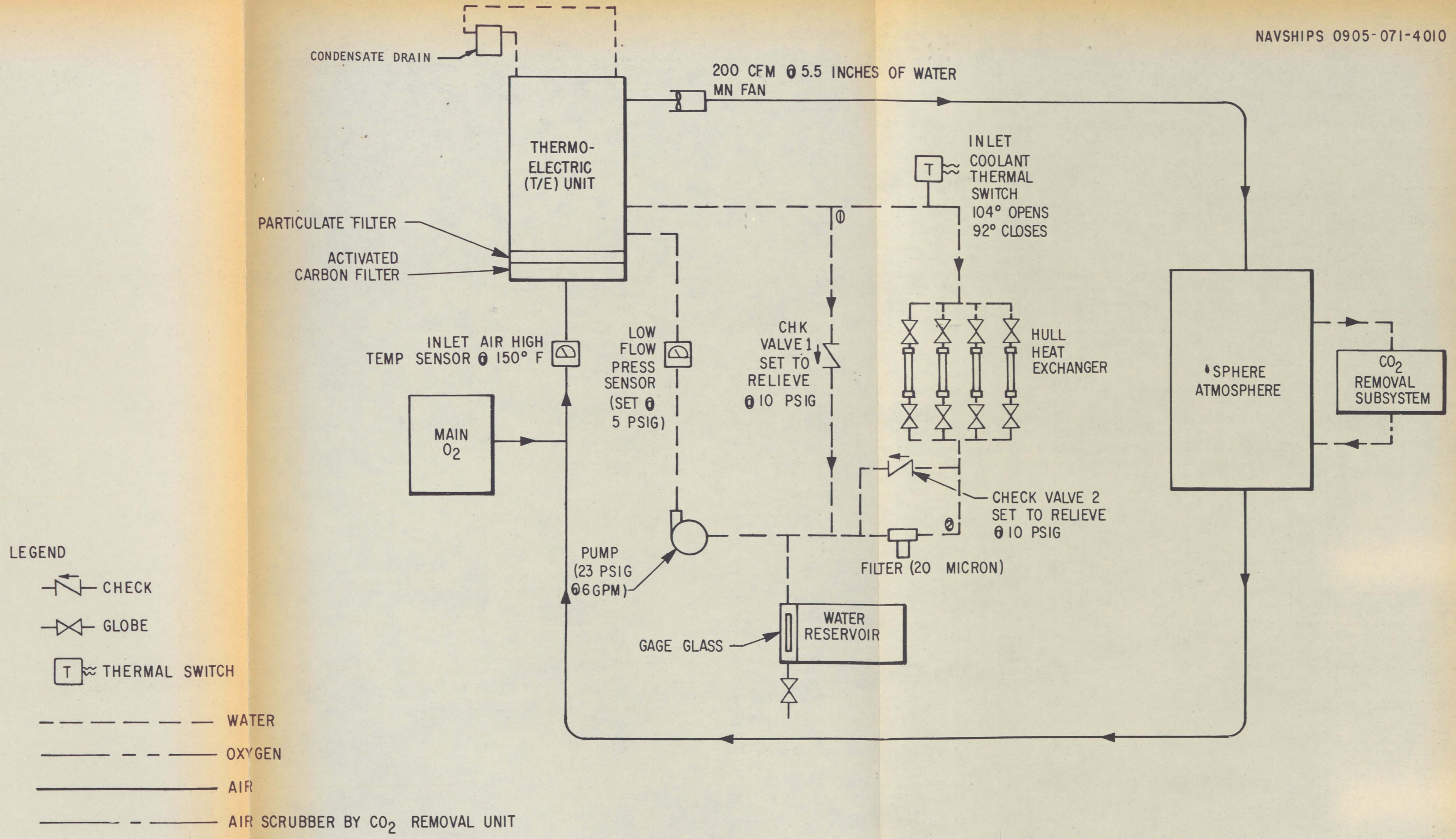
FIGURE 5-1. LIFE SUPPORT SYSTEM WITH THERMOELECTRIC UNIT
