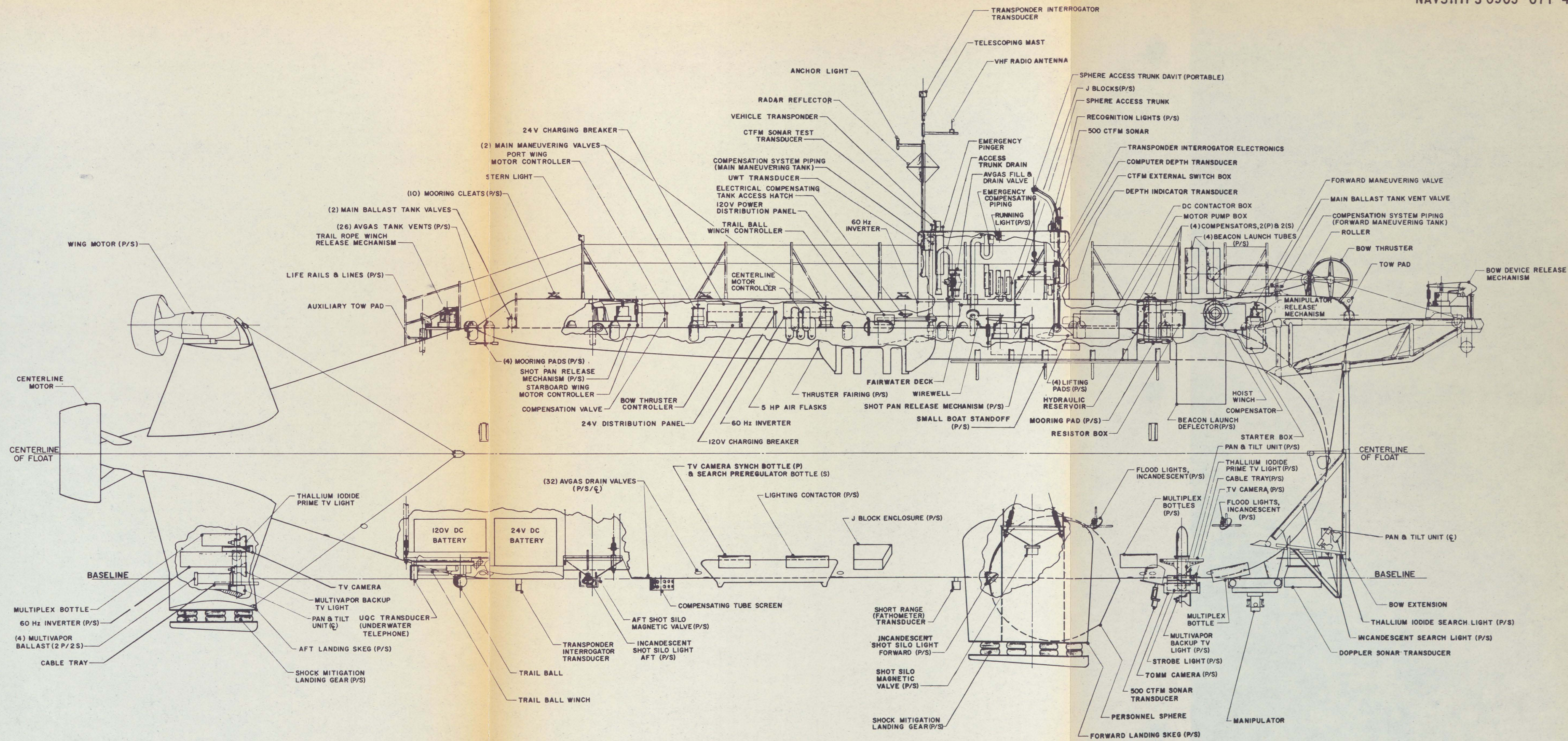
FIGURE I-2. TRIESTE II (DSV-I) EQUIPMENT CONFIGURATION
