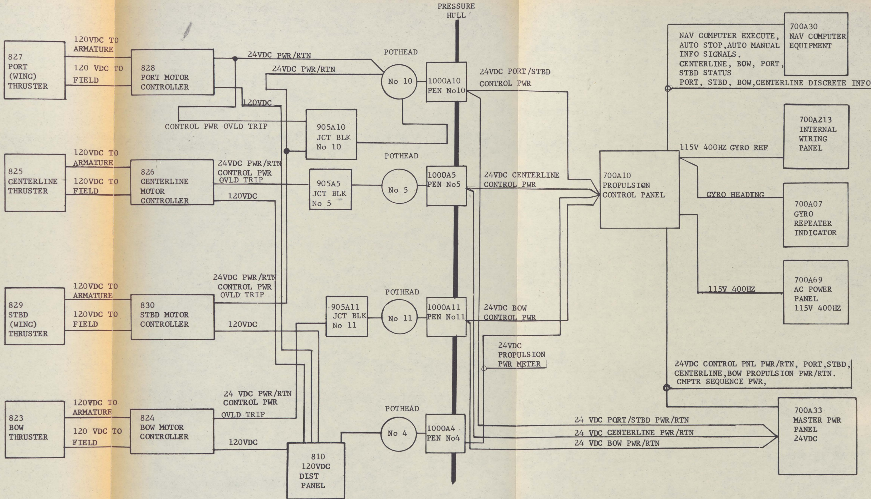
FIGURE 3-10. PROPULSION SYSTEM POWER AND CONTROL DIAGRAM
