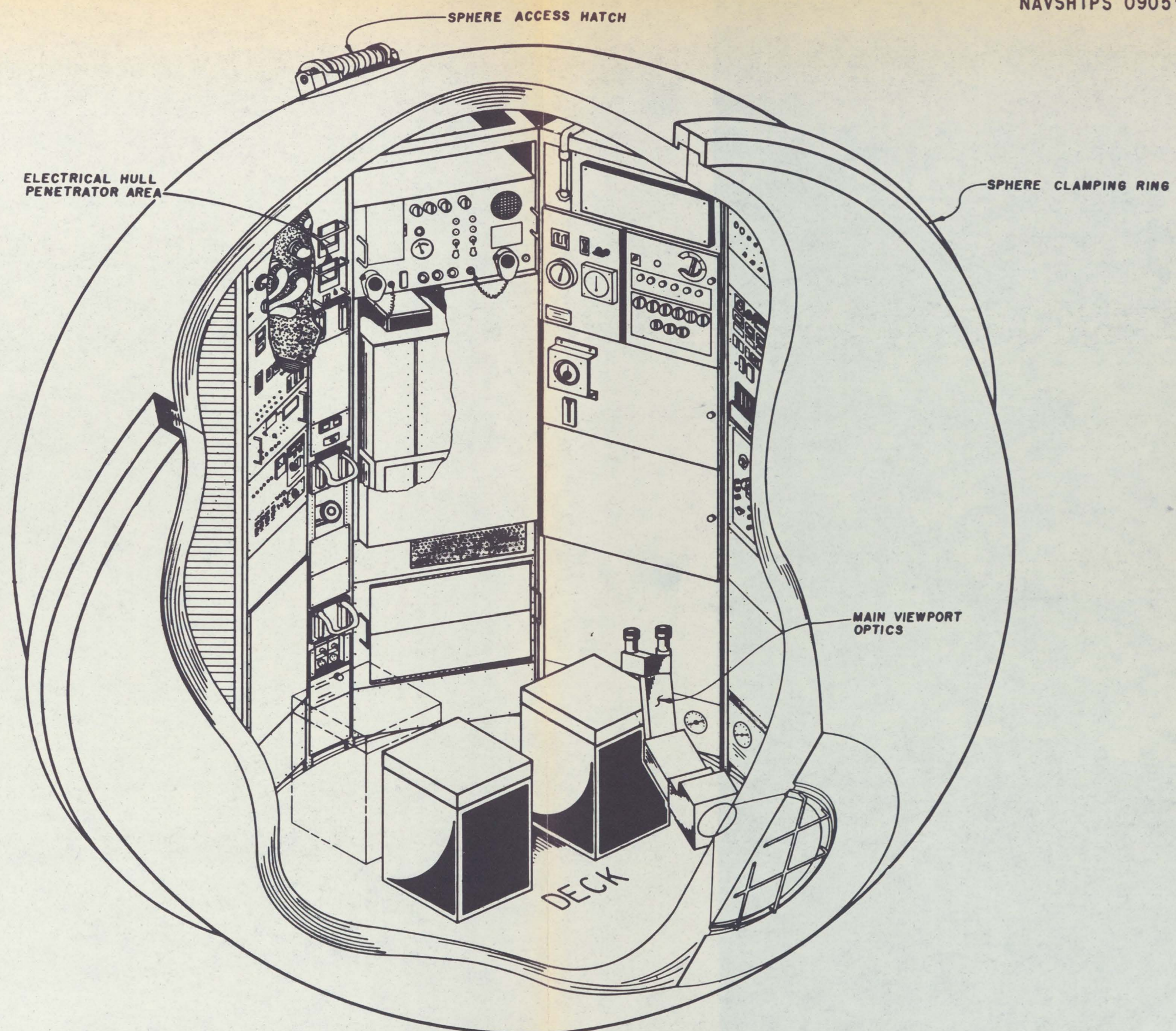
FIGURE 1-3. PERSONNEL SPHERE
