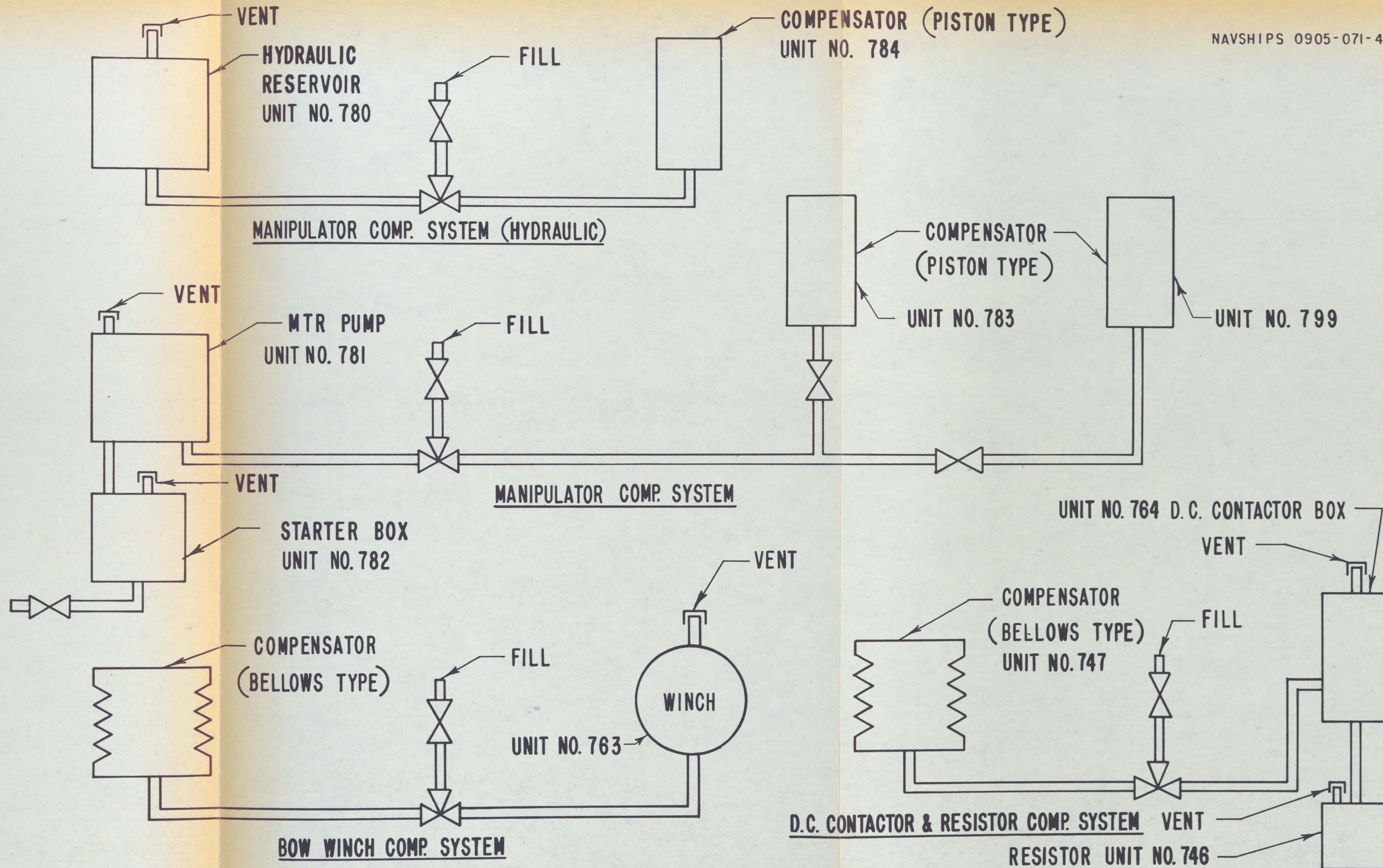
FIGURE 2-9. APPENDAGE COMPENSATION SYSTEM
