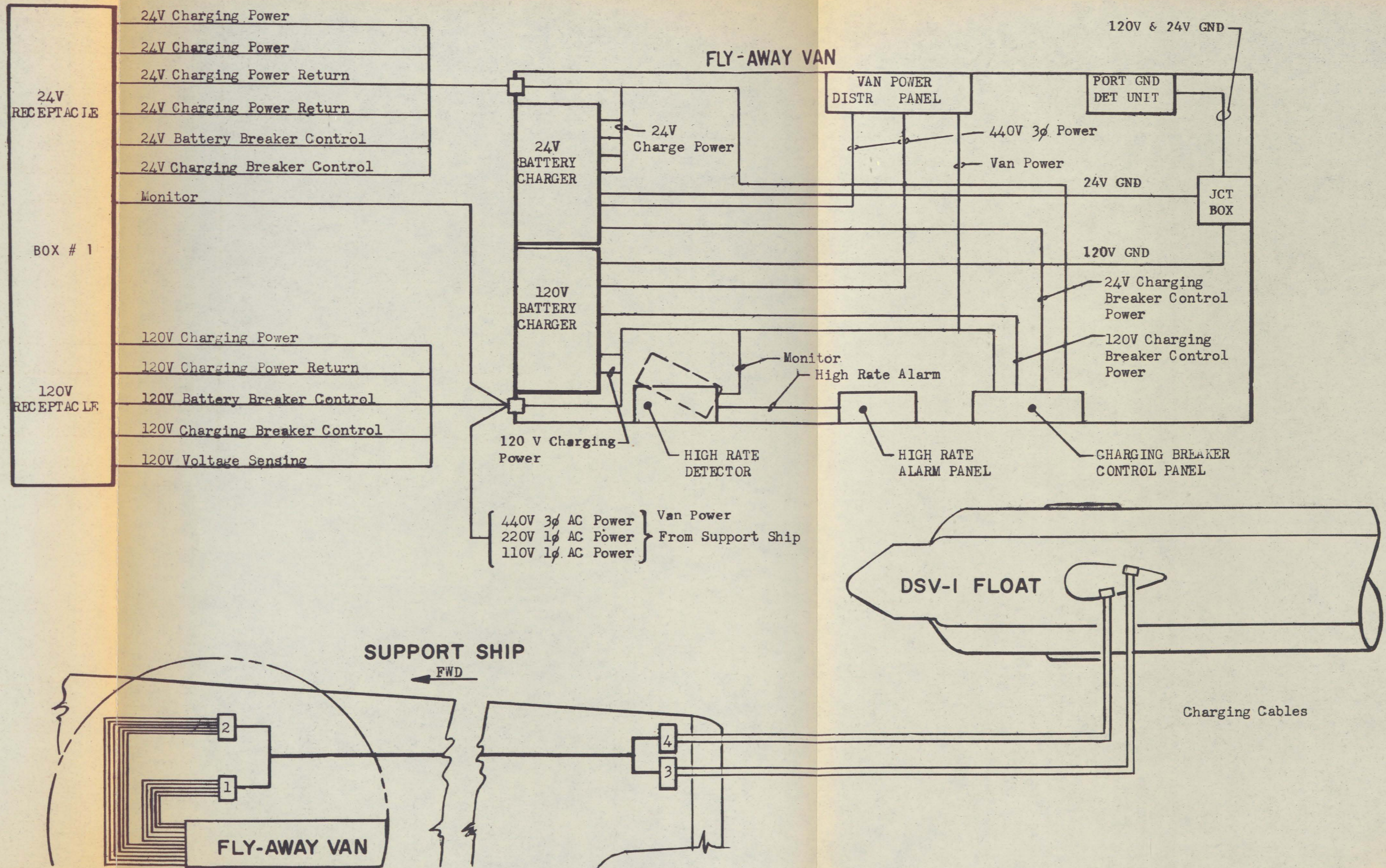
FIGURE 7-10. BATTERY CHARGING FACILITY AND CABLING
