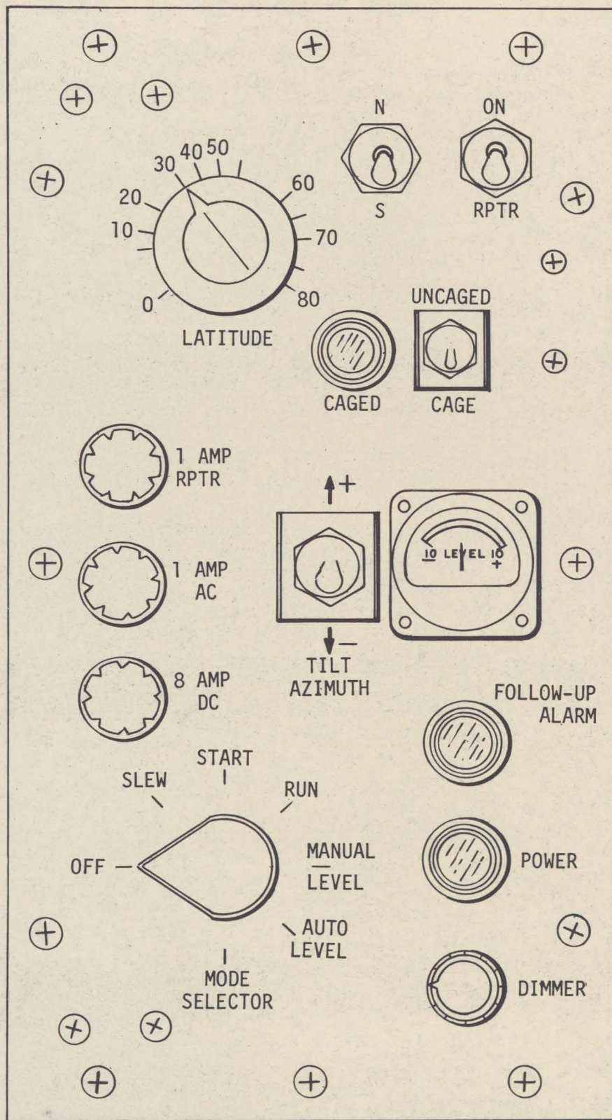
FIGURE 4-II. GYROCOMPASS CONTROL PANEL
