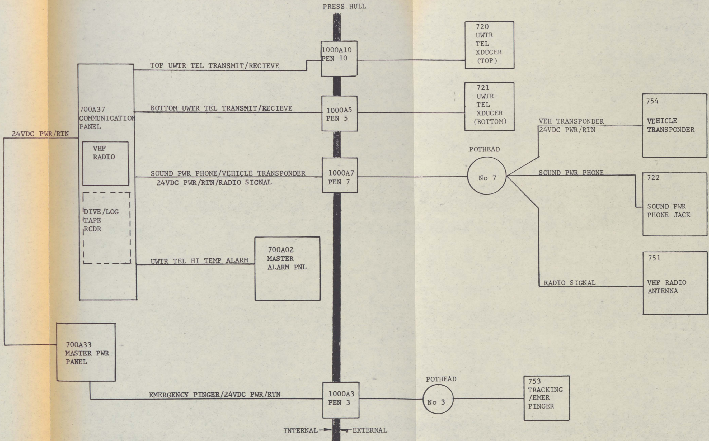
FIGURE 4-24. COMMUNICATIONS SYSTEM
