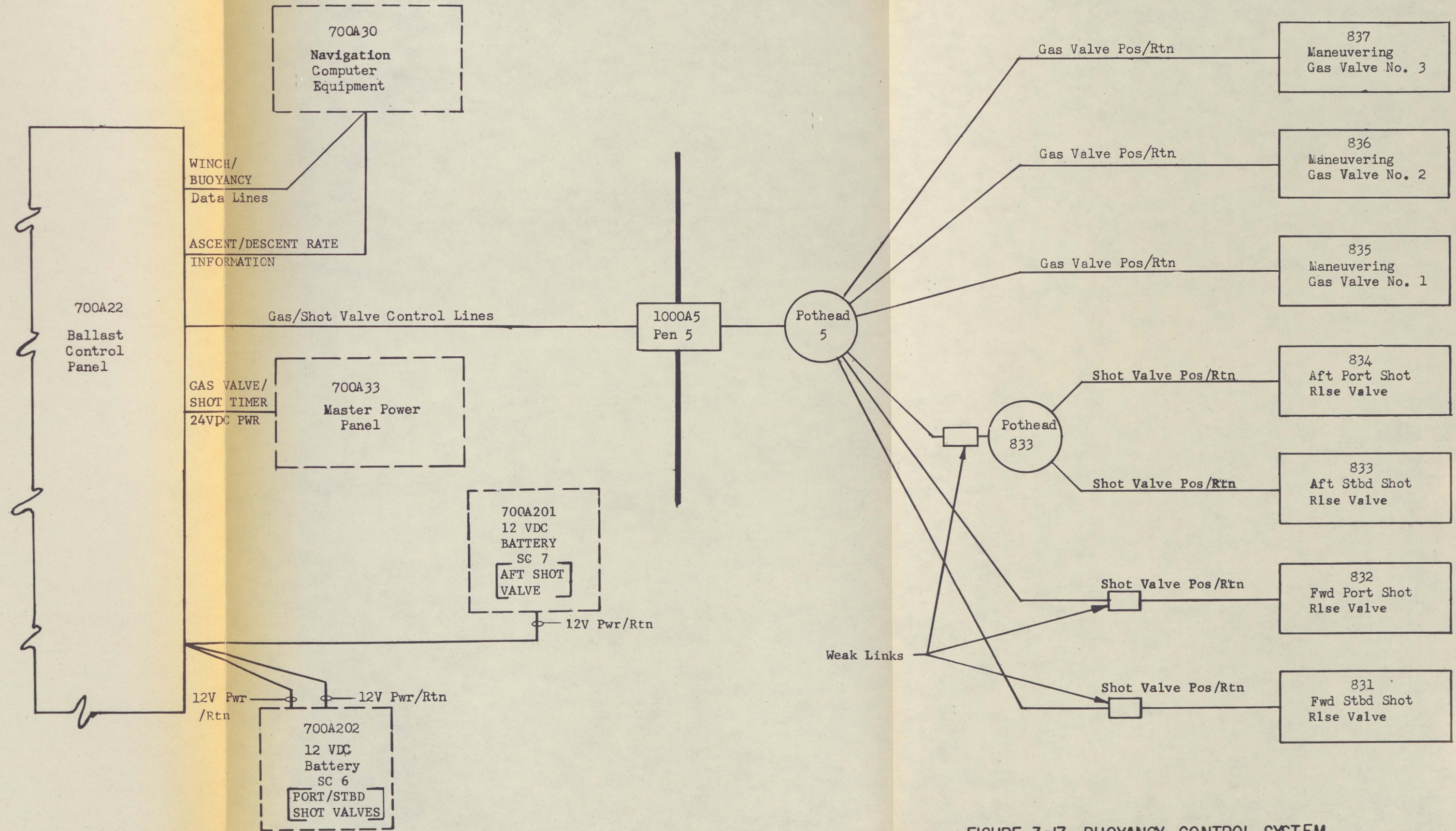
FIGURE 3-17. BUOYANCY CONTROL SYSTEM
