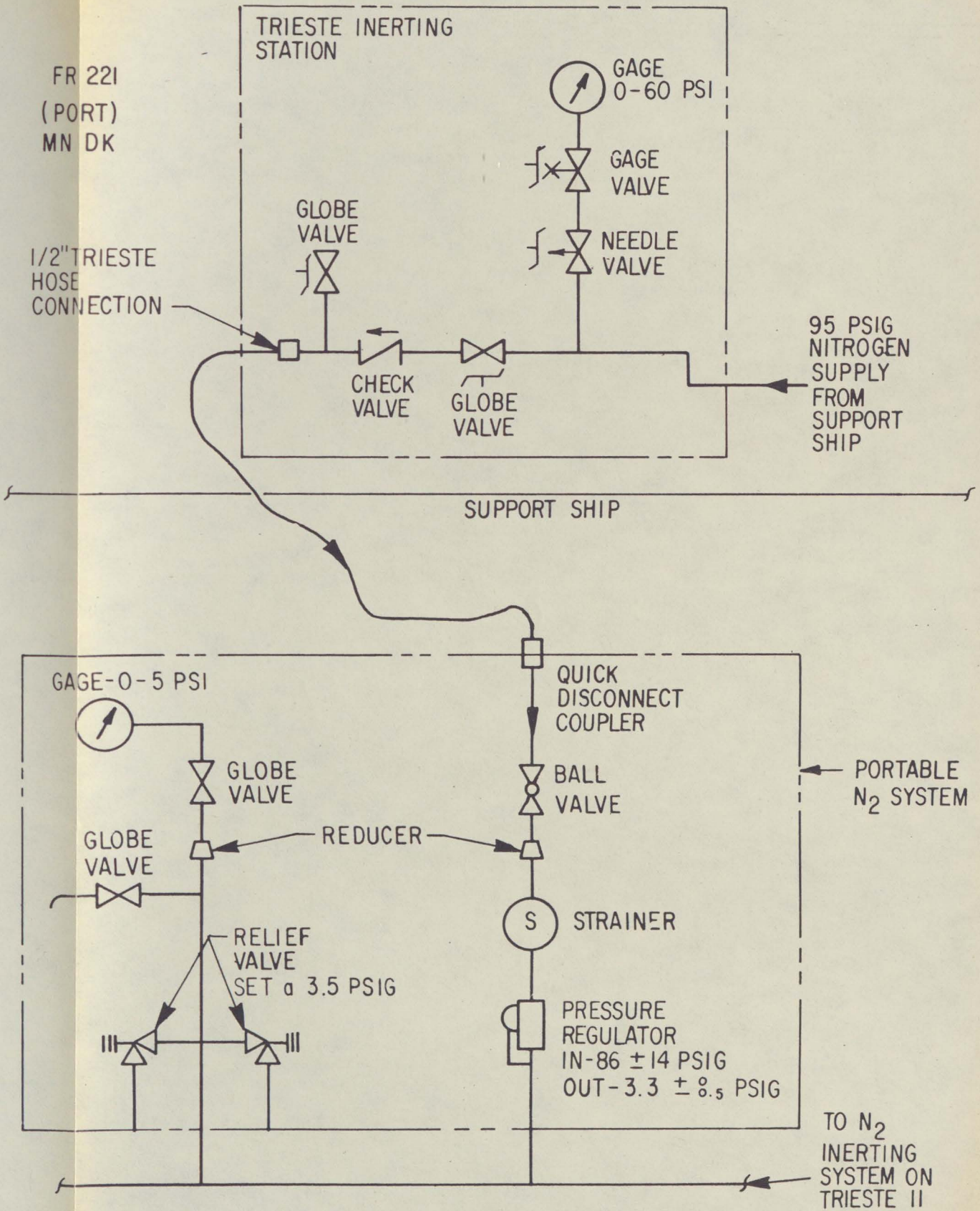
FIGURE 7-8. NITROGEN SYSTEM INTERFACE
