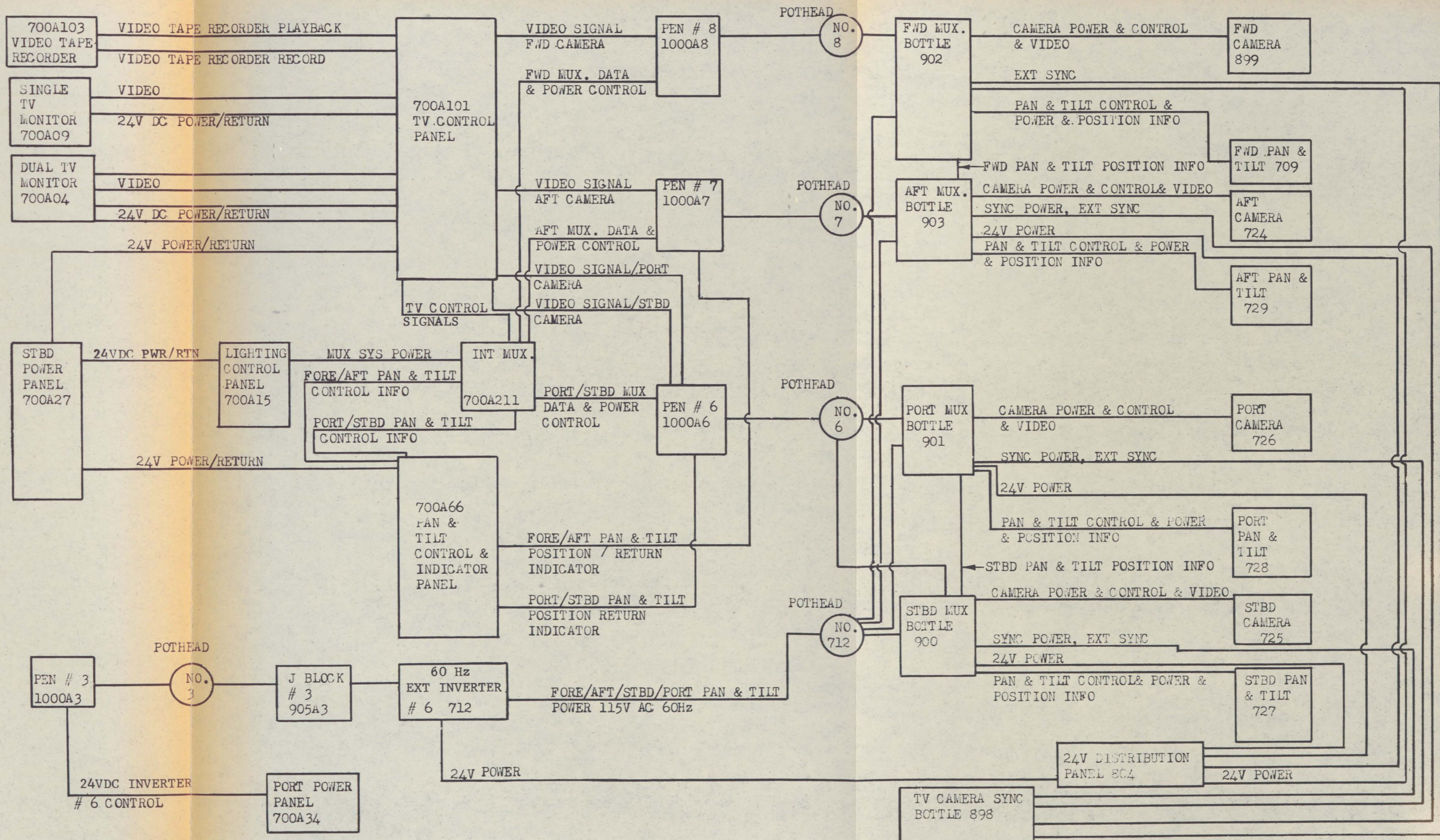
FIGURE 4-26. TV SYSTEM
